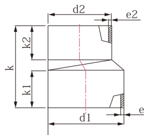
Eccentric Reducer
