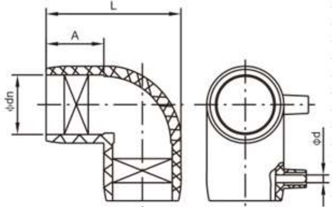
Electrofusion Elbow 90°
