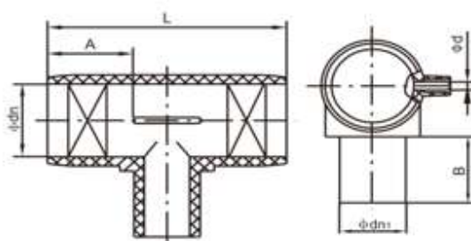
Electrofusion Reducing Tee
