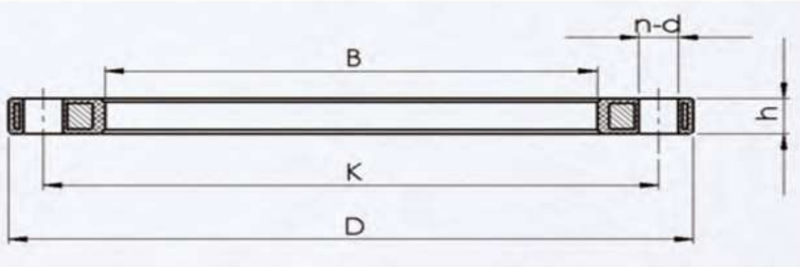
PP - Steel Flange Plate Pn 10
