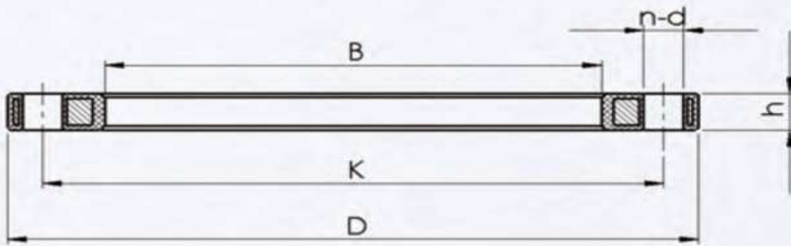
PP - Steel Flange Plate Pn 16
