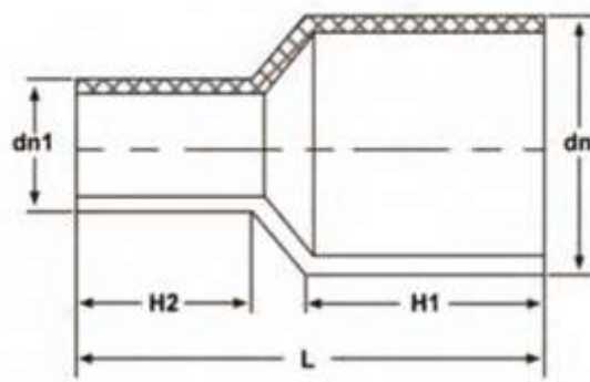
Reducer 1
