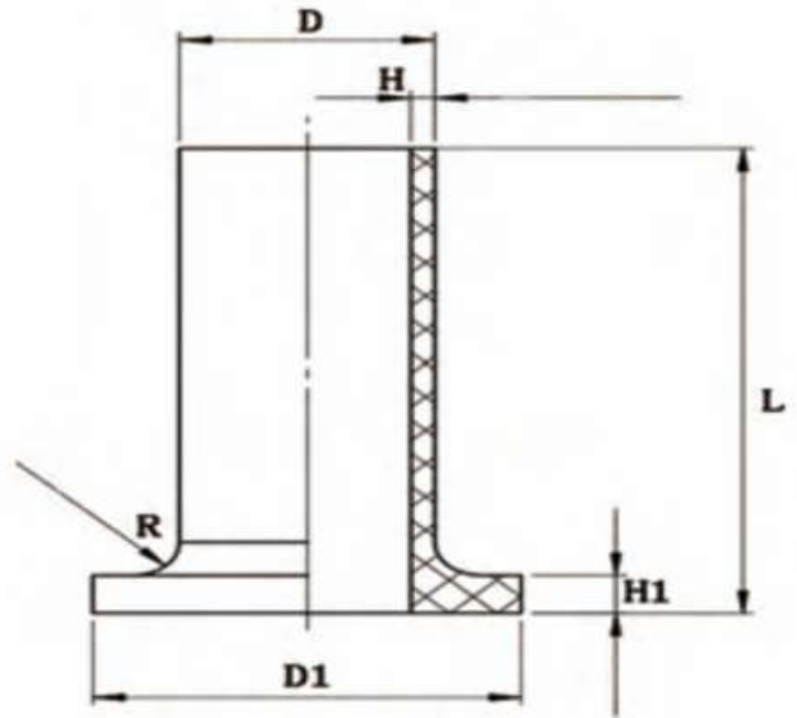
Stub End 2
